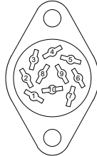
Camera Interface 10 pin Jack
