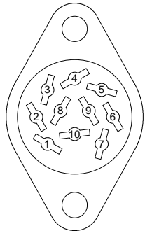
Camera Interface 10 pin DIN Jack Front View
