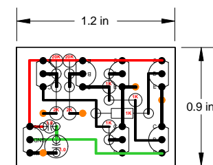
Perf Board Layout of Remote Focus Motor Driver
